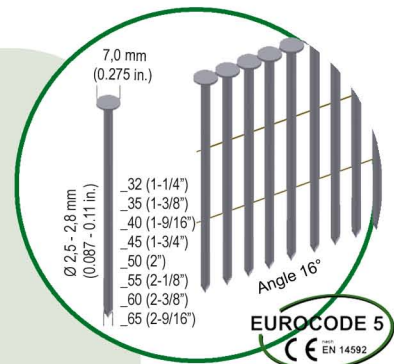
Coilnails CNW wire collated
