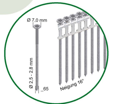
Nail screws CSS plastic collated - sheet bounded for residue-free processing
