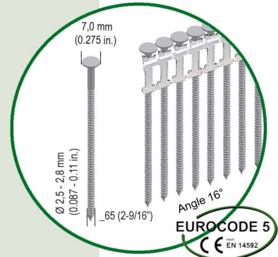
Coilnails CNS plastic collated - sheet bounded for residue-free processing
